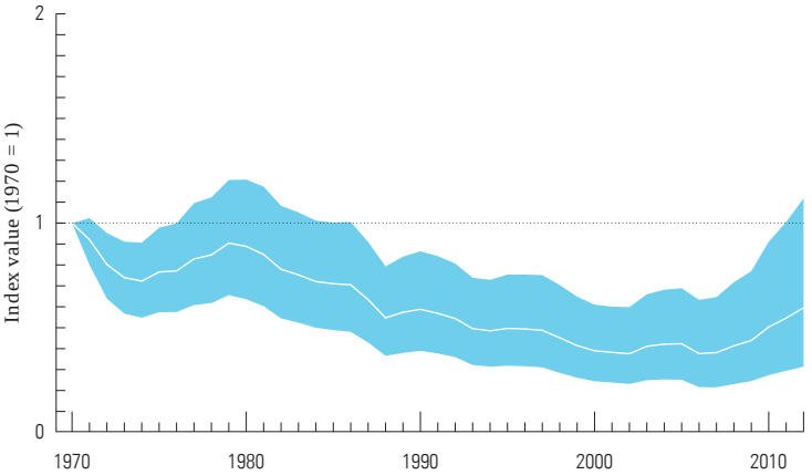
Figure 17: The migratory fish LPI shows a decline of 41 per cent (range: +12 to -69 per cent) between 1970 and 2012. Trend in population abundance for 735 populations of 162 migratory fish species monitored worldwide between 1970 and 2012 (WWF/ZSL, 2016). The species included in this index are classified as either catadromous, anadromous, potamodromous or amphidromous by GROMS (Global Register of Migratory Species).
