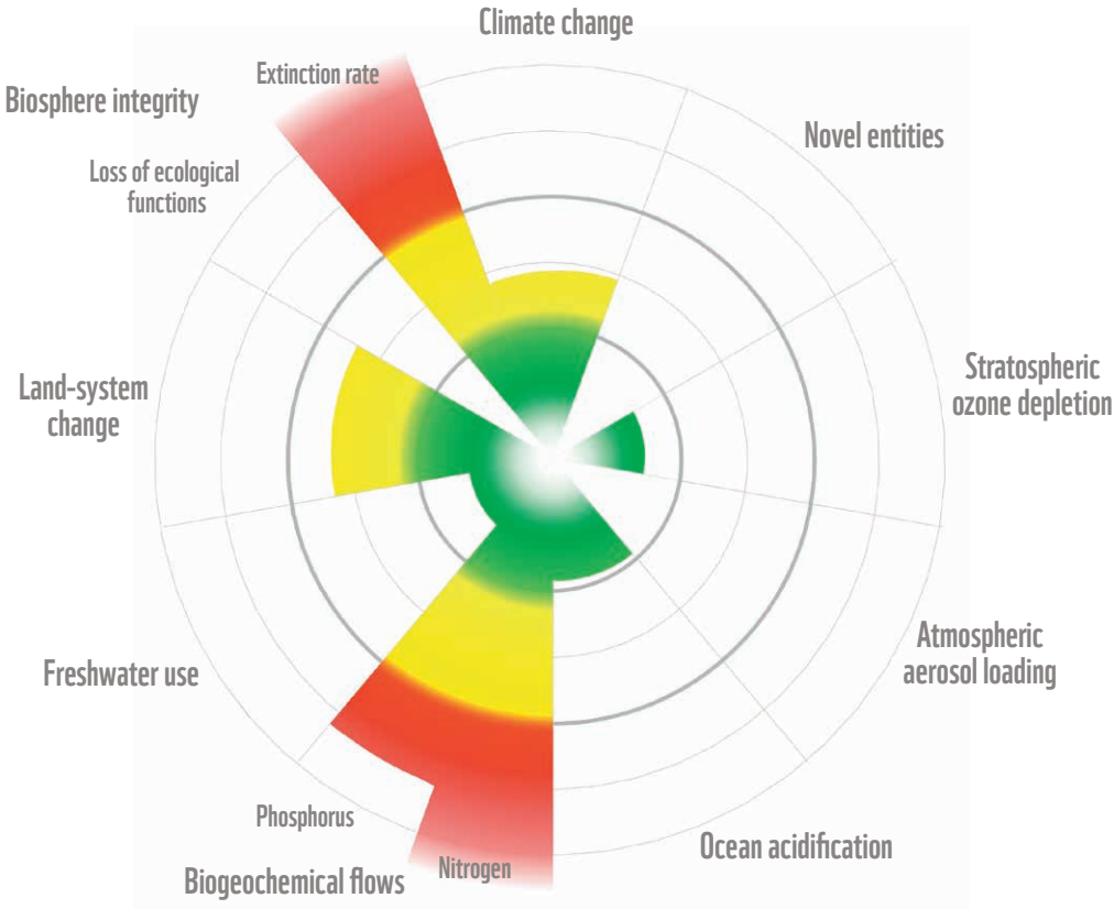
Figure 30: Planetary Boundaries The green zone is the safe operating space (below the boundary), yellow represents the zone of uncertainty, with an increasing risk of disrupting Earth system stability; and red is the high-risk zone, pushing the Earth system out of a stable Holocene-like state. The Planetary Boundary itself lies at the inner heavy circle (Steffen et al., 2015).
