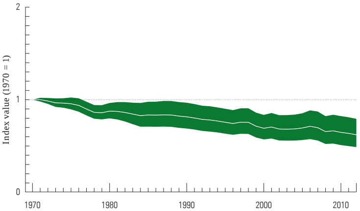
Figure 5: The terrestrial LPI shows a decline of 38 per cent (range: -21 to -51 per cent) between 1970 and 2012 Trend in population abundance for 4,658 populations of 1,678 terrestrial species monitored across the globe between 1970 and 2012 (WWF/ZSL, 2016).
