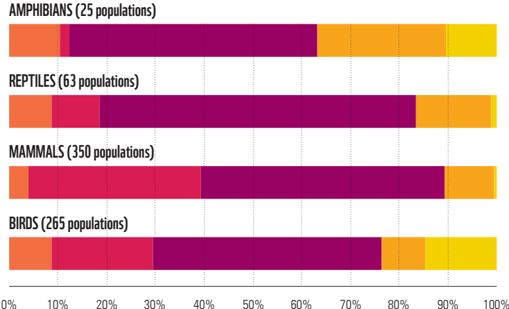
Figure 7: Taxonomic differences in threat frequency for 703 declining terrestrial populations in the LPI database (WWF/ZSL, 2016).
